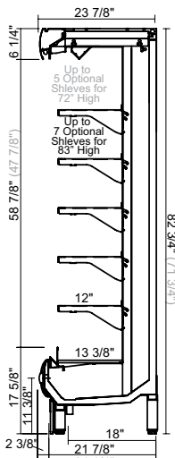
RGD24 83 and RGD24 72
