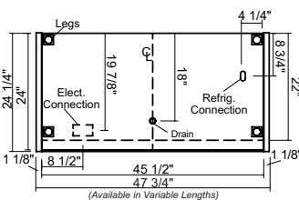
RGD 24 Wide Plan View
