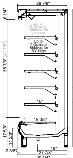
RGD30 83 and RGD30 72
