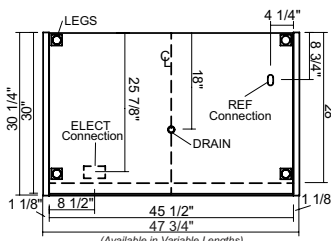
RGD 30 Wide Plan View
